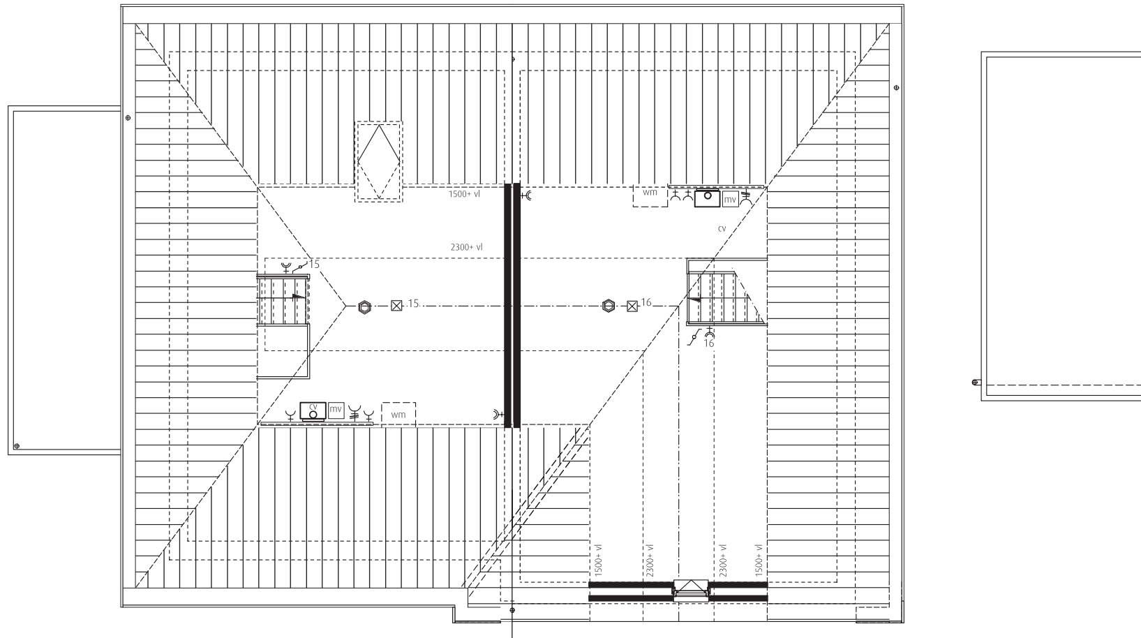
zolder [schaal 1:100]
