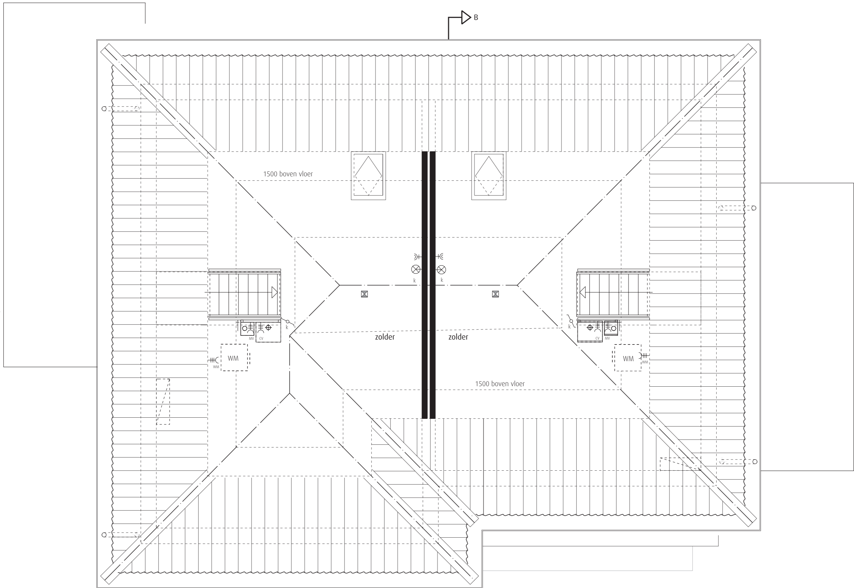
Beukenhaege zolder [schaal 1:50]
